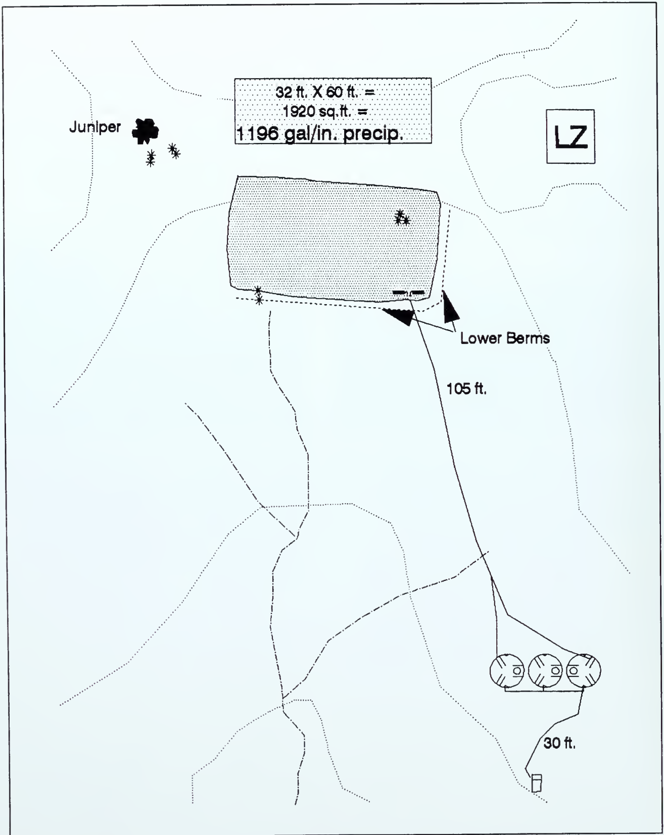
Figure 3. Badger apron water development; example of a hypalon apron setup.
